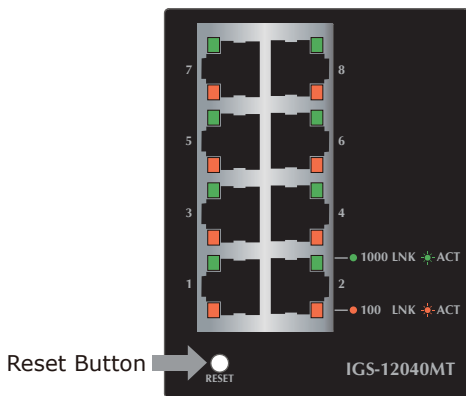
Figure 6-3: IGS-12040MT Reset Button
