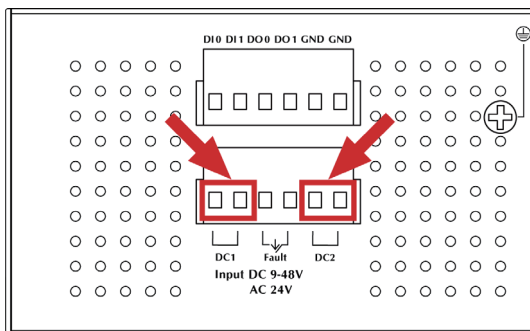
Figure 3-4: IGS-20040MT Upper Panel
