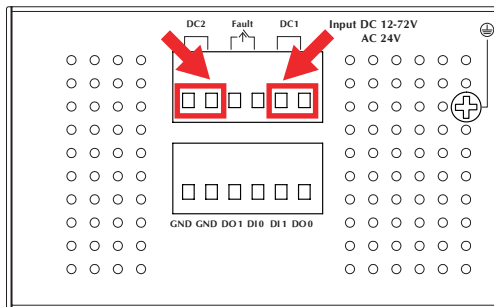
Figure 3-3: IGS-12040MT Upper Panel
