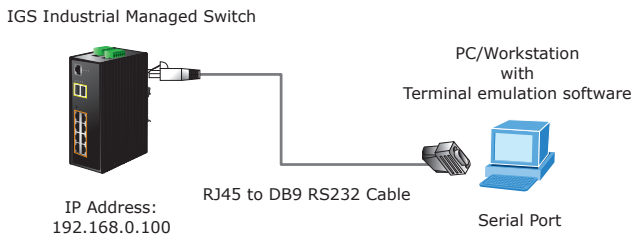
Figure 4-1: Industrial L2+ Managed Switch Console Connectivity
