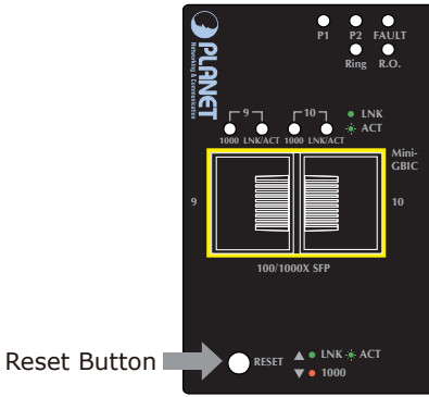
Figure 6-1: IGS-10020MT Reset Button
