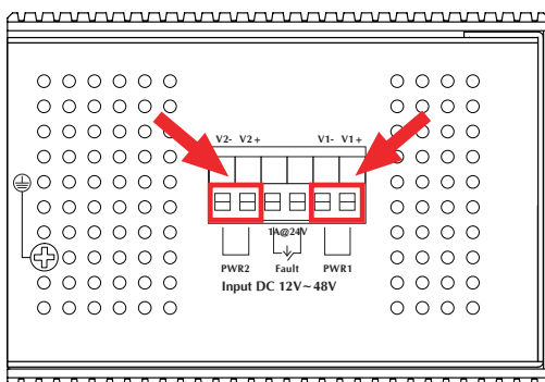
Figure 3-2: IGS-10080MFT Upper Panel
