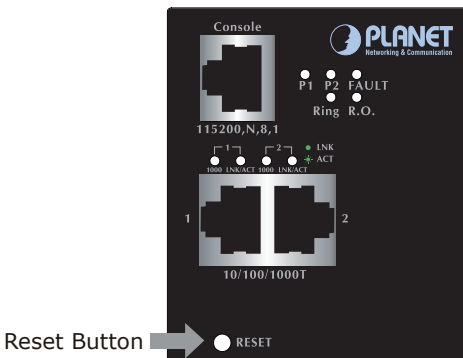
Figure 6-2: IGS-10080MFT Reset Button
