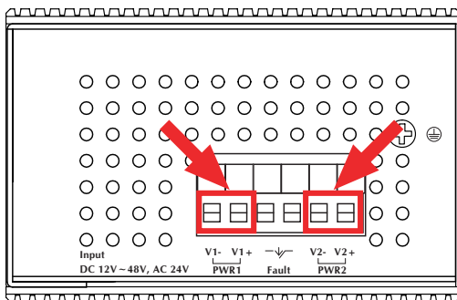
Figure 3-1: IGS-10020MT Upper Panel
